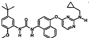
1-(5-tert-Butyl-2-methoxy-phenyl)-3-{4-[2-(cyclopropylmethyl-amino)-pyrimidin-4-yloxy]-naphthalen-1-yl}-urea;
